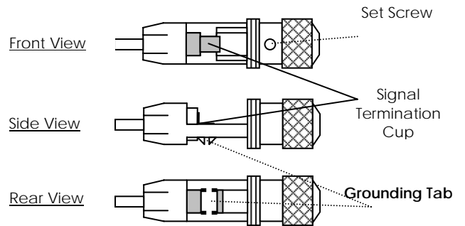
Diagram 2: Connector Overview
